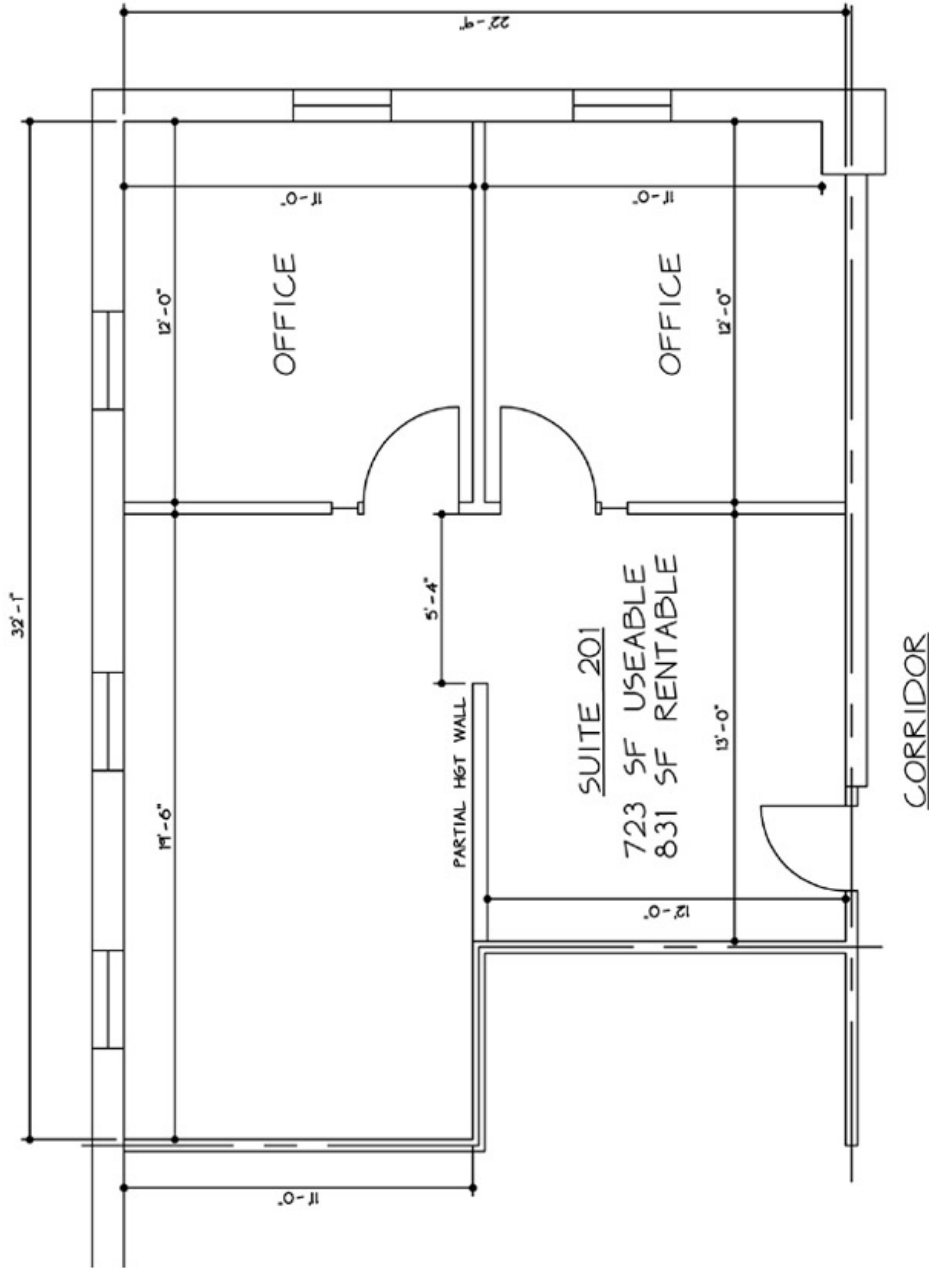
FLOOR PLAN 1/4"=1'-0"
